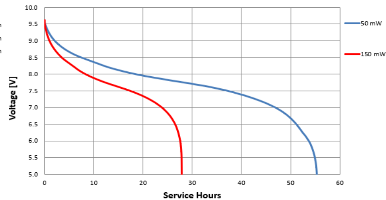
Constant Power
